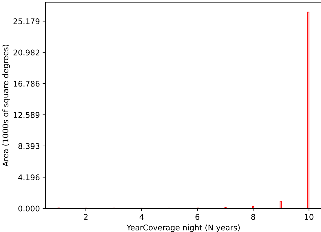
too_ignore_10_1v3.4_10yrs i band: YearCoverage night
