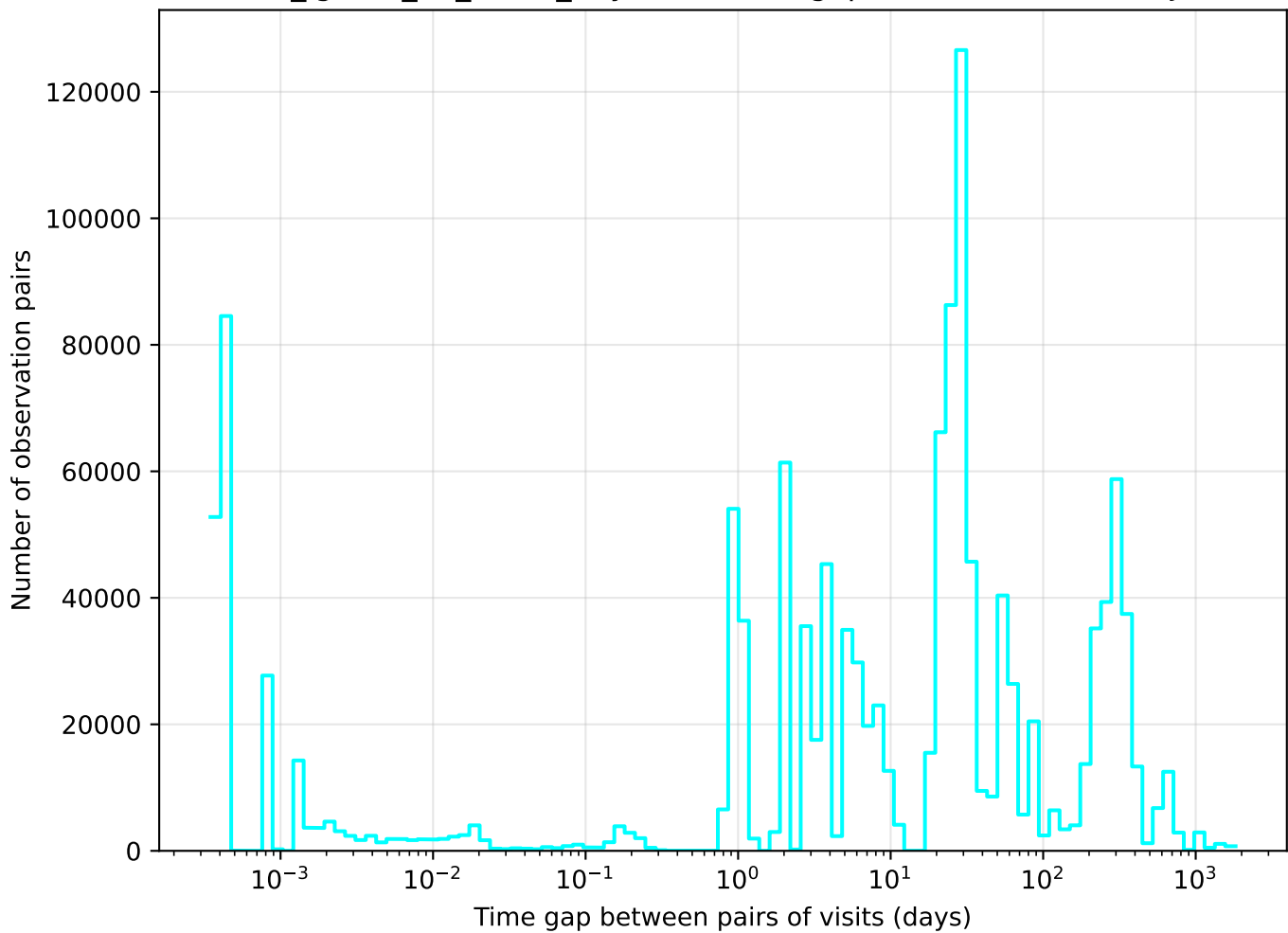
too_ignore_10_1v3.4_10yrs u band: Tgaps observationStartMJD
