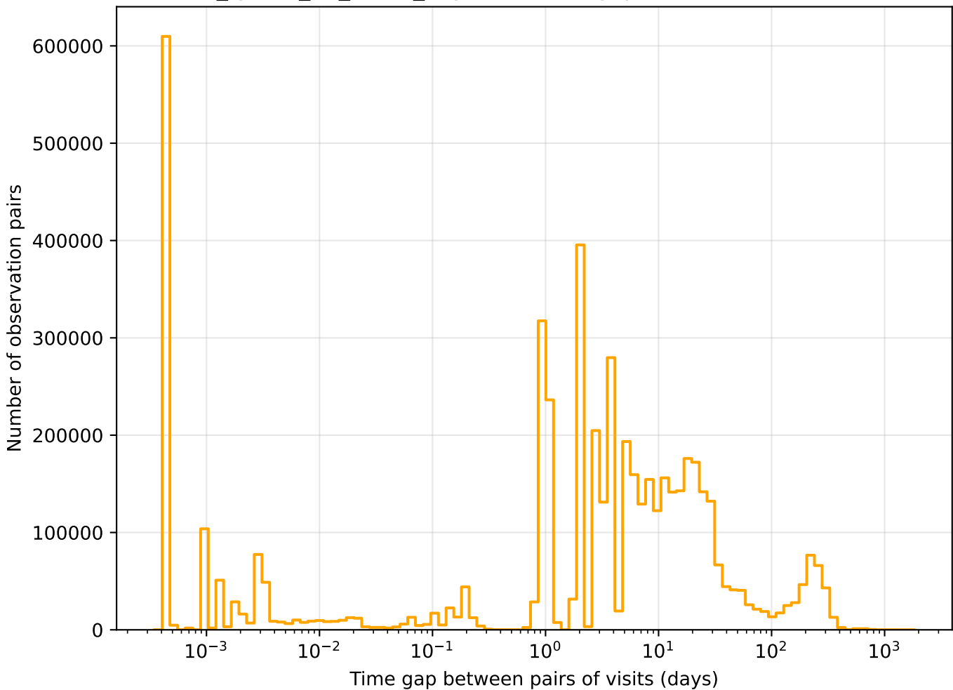
too_ignore_10_1v3.4_10yrs r band: Tgaps observationStartMJD
