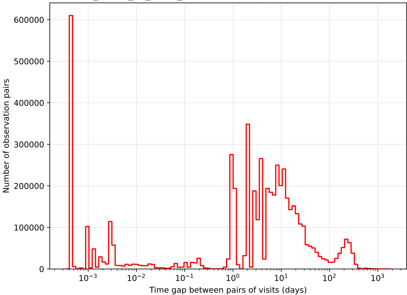
too_ignore_10_1v3.4_10yrs i band: Tgaps observationStartMJD
