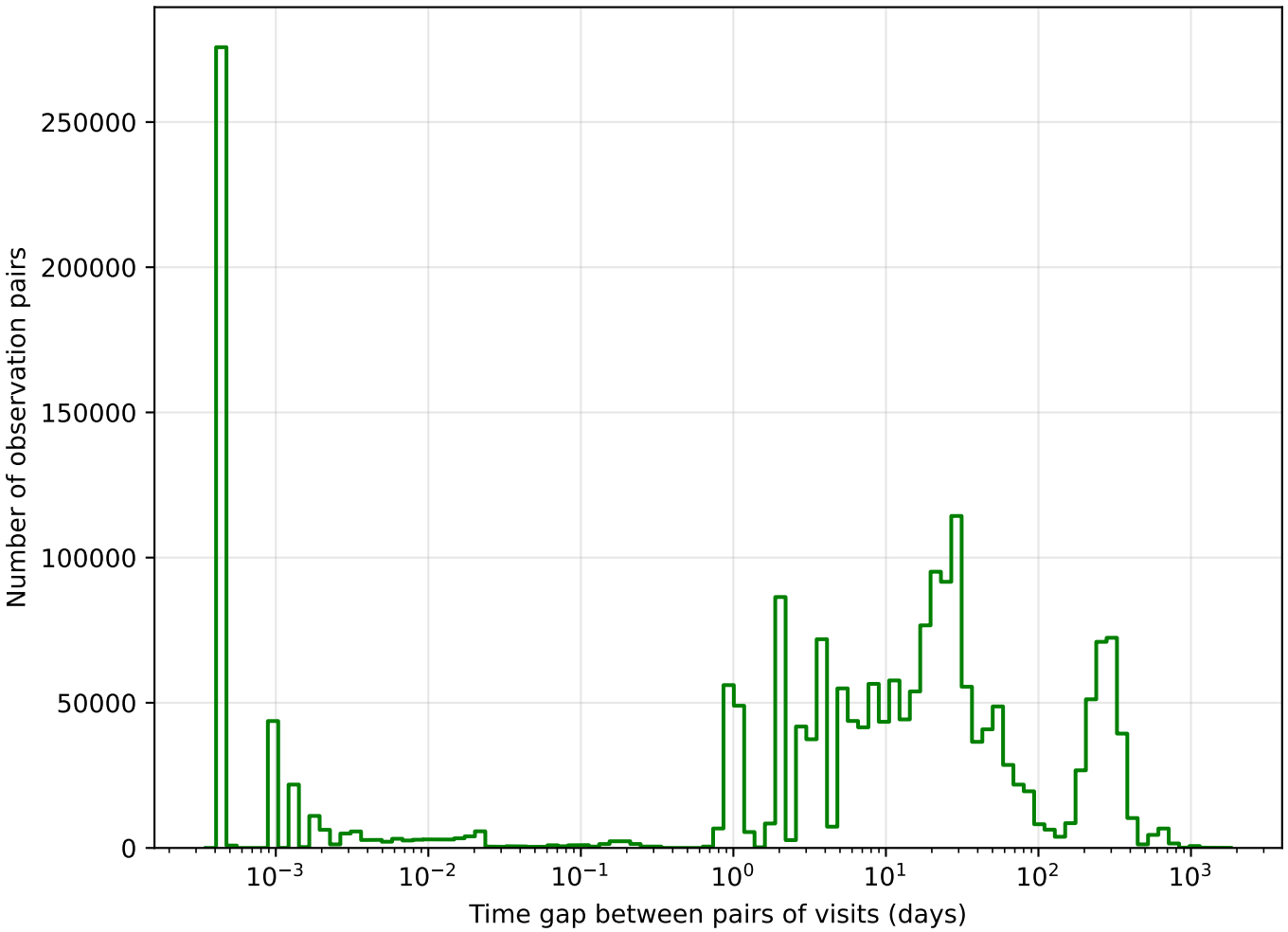
too_ignore_10_1v3.4_10yrs g band: Tgaps observationStartMJD
