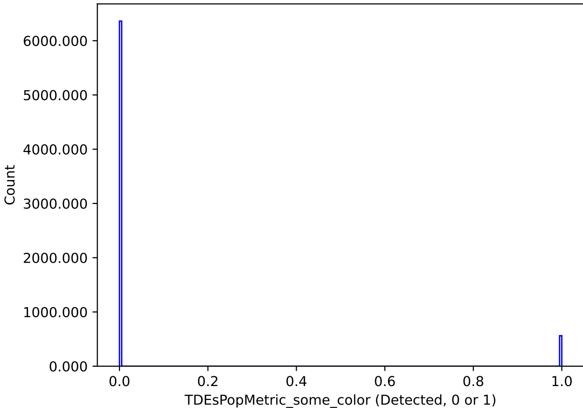
too_ignore_10_1v3.4_10yrs : TDEsPopMetric_some_color
