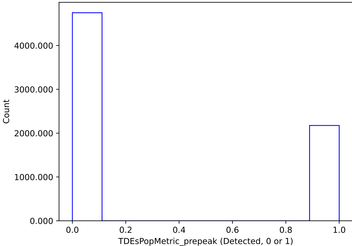
too_ignore_10_1v3.4_10yrs : TDEsPopMetric_prepeak
