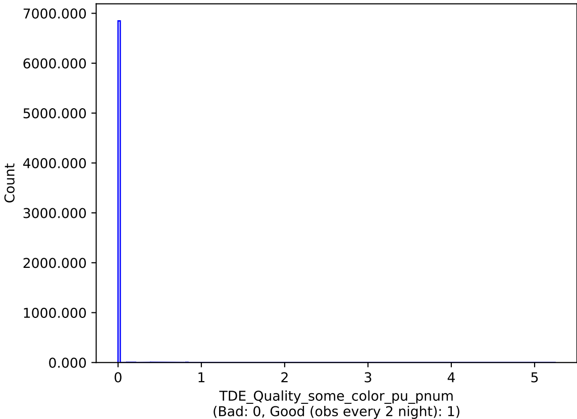
too_ignore_10_1v3.4_10yrs : TDE_Quality_some_color_pu_pnum
