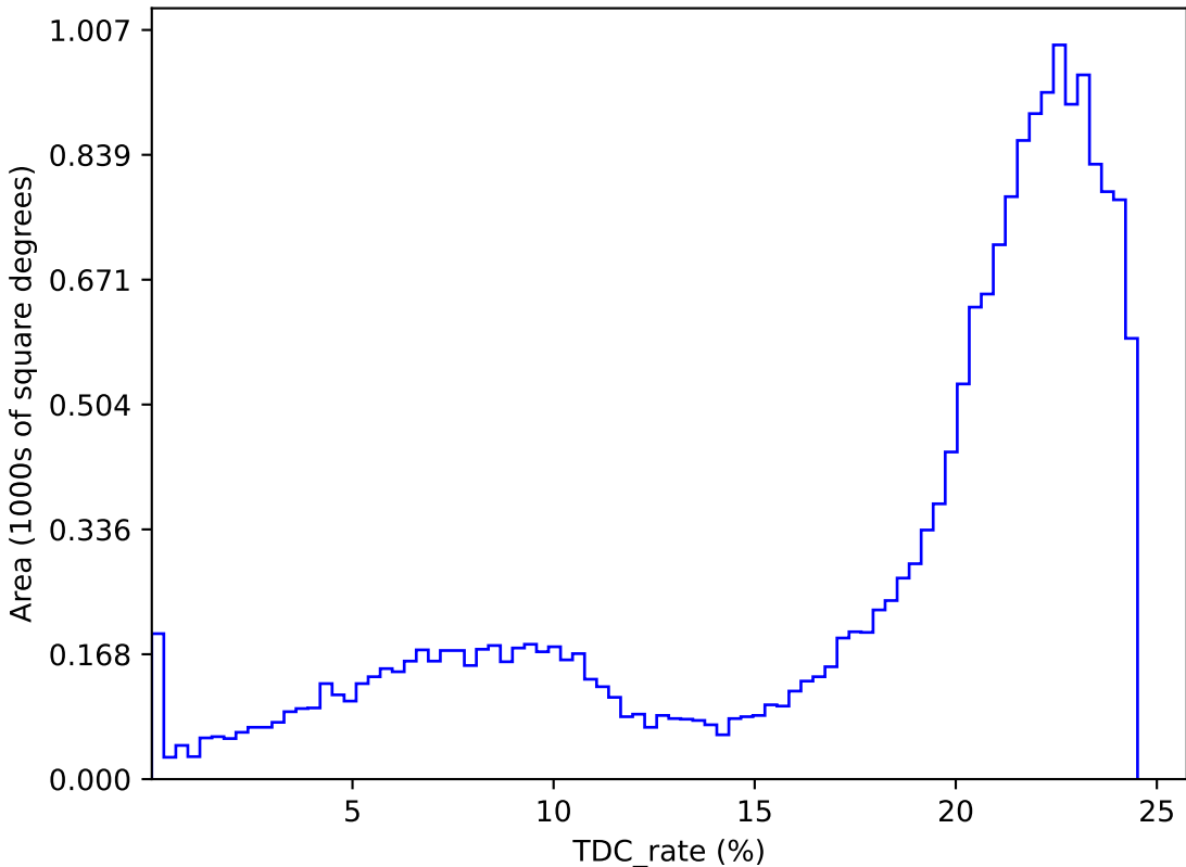
too_ignore_10_1v3.4_10yrs : TDC_rate
