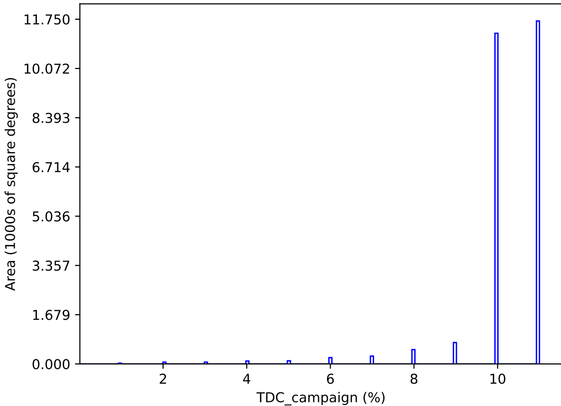
too_ignore_10_1v3.4_10yrs : TDC_campaign
