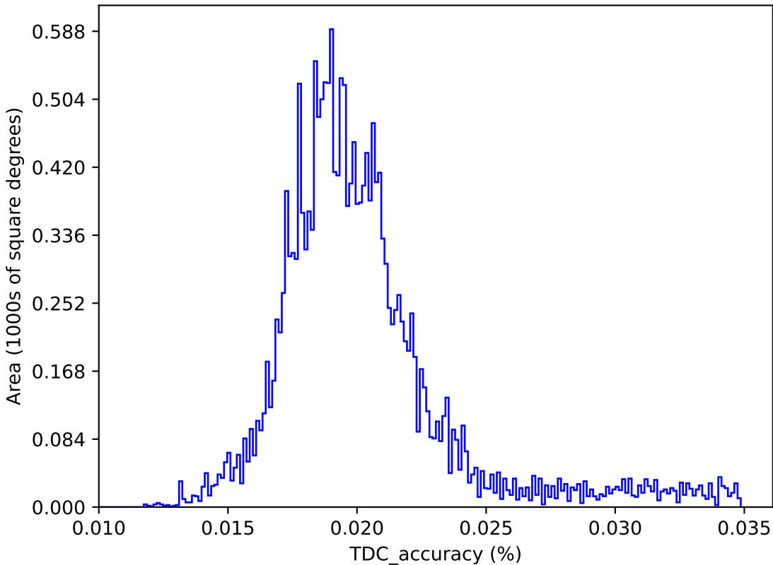
too_ignore_10_1v3.4_10yrs : TDC_accuracy
