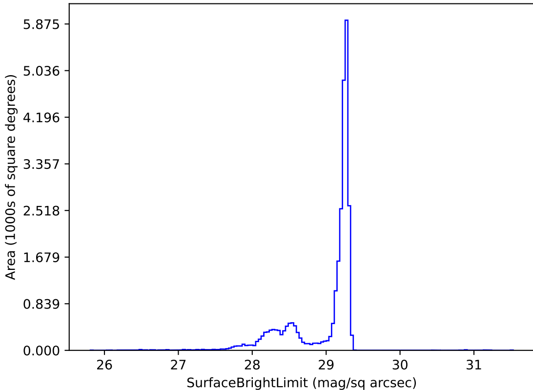
too_ignore_10_1v3.4_10yrs z: SurfaceBrightLimit
