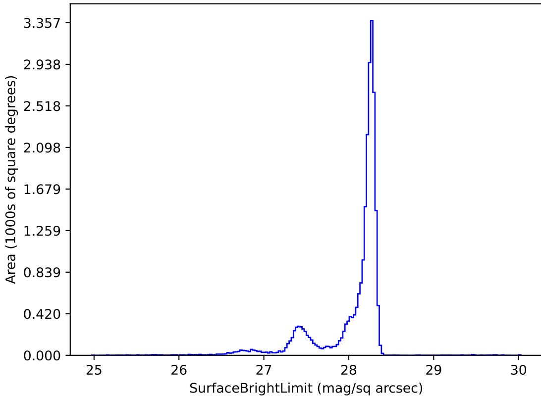
too_ignore_10_1v3.4_10yrs y: SurfaceBrightLimit
