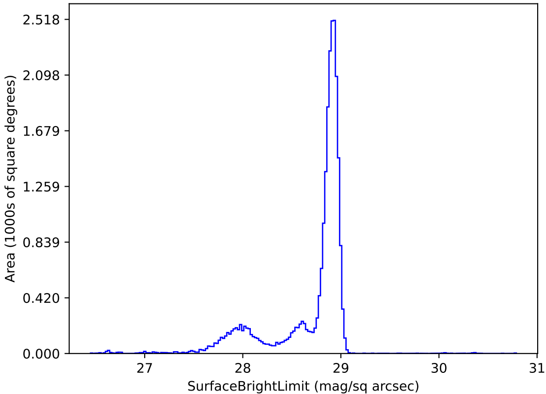
too_ignore_10_1v3.4_10yrs u: SurfaceBrightLimit
