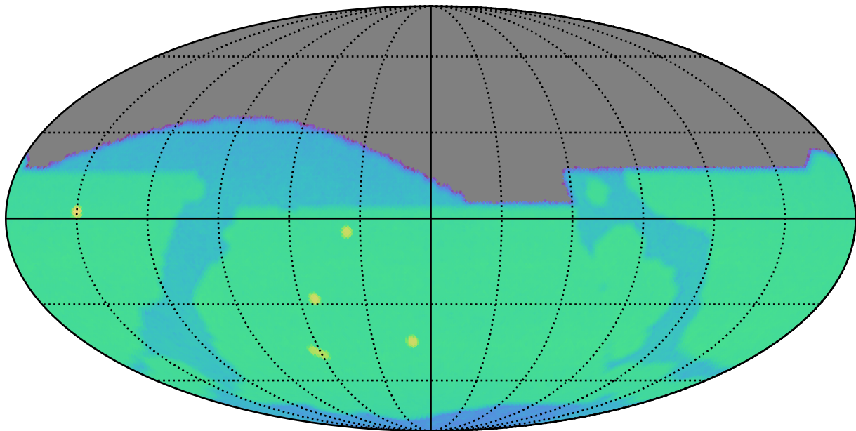
too_ignore_10_1v3.4_10yrs i: SurfaceBrightLimit
