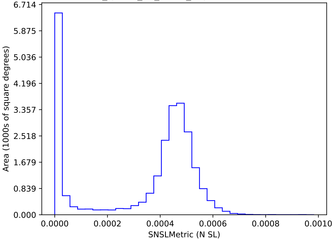
too_ignore_10_1v3.4_10yrs : SNSLMetric
