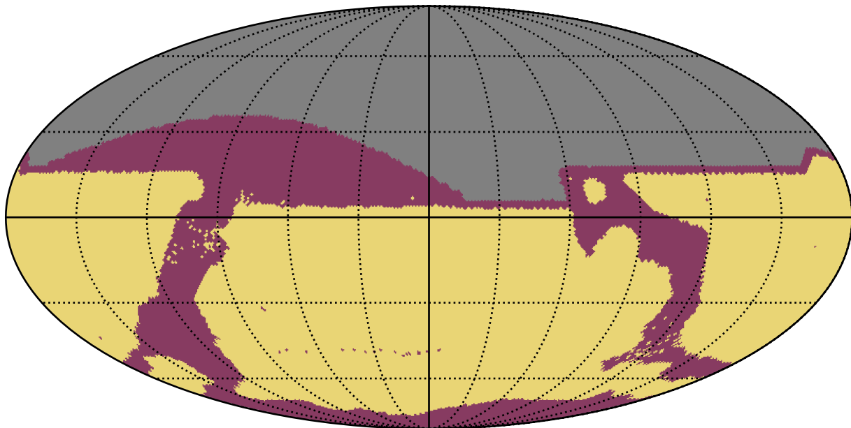
too_ignore_10_1v3.4_10yrs : RapidRevisits
