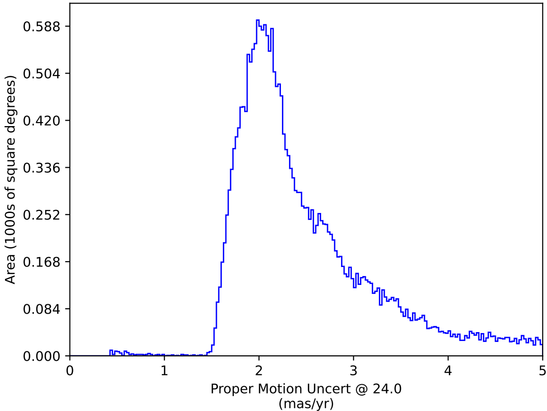
too_ignore_10_1v3.4_10yrs : Proper Motion Uncert @ 24.0
