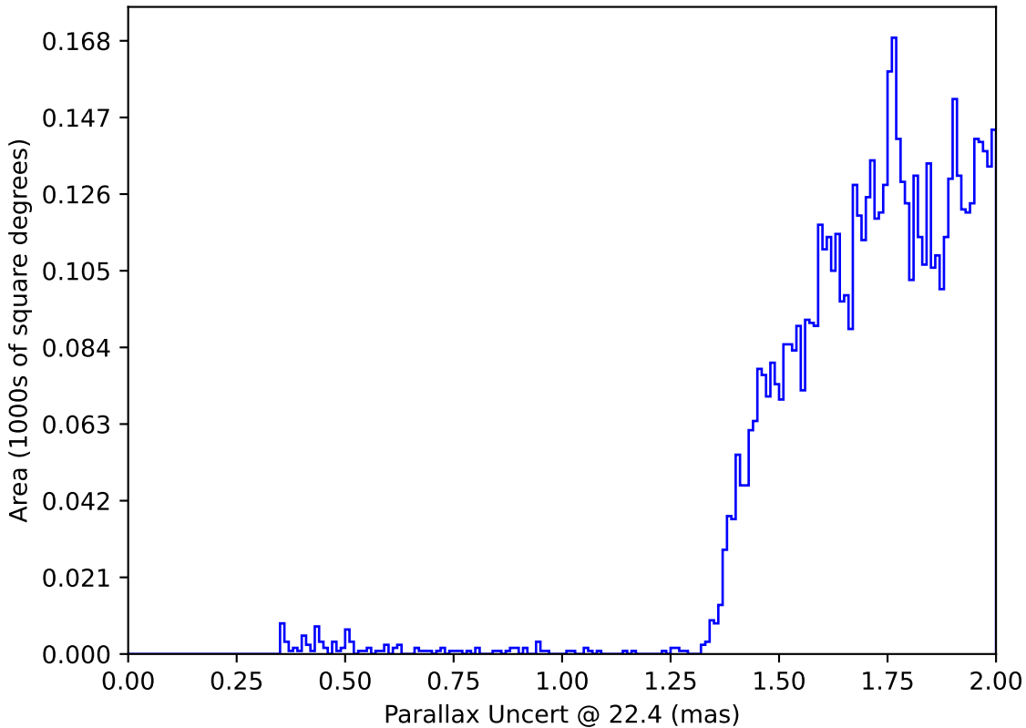
too_ignore_10_1v3.4_10yrs : Parallax Uncert @ 22.4
