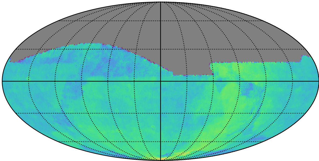
too_ignore_10_1v3.4_10yrs : Parallax Coverage @ 24.0
