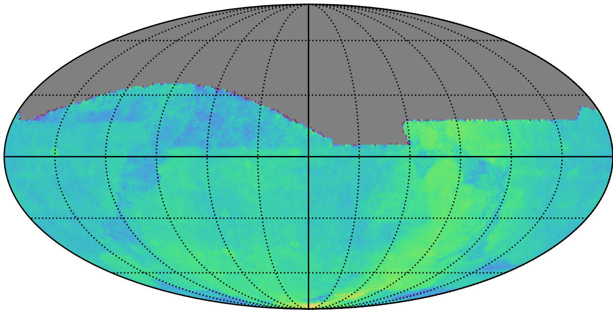
too_ignore_10_1v3.4_10yrs : Parallax Coverage @ 22.4
