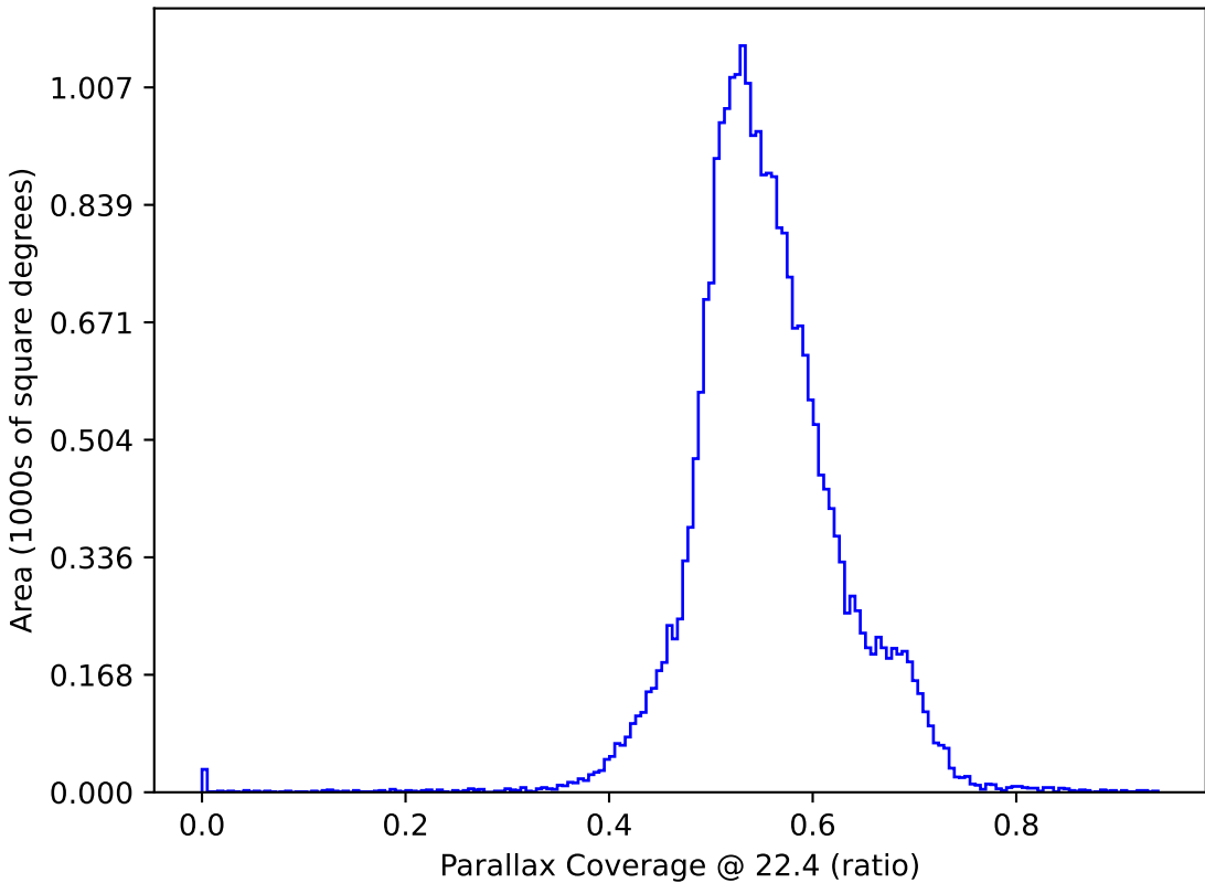
too_ignore_10_1v3.4_10yrs : Parallax Coverage @ 22.4
