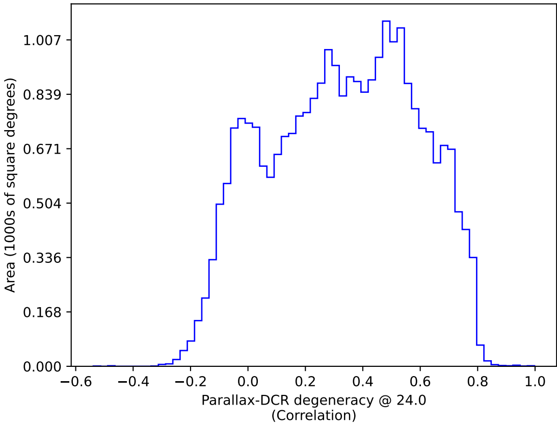
too_ignore_10_1v3.4_10yrs : Parallax-DCR degeneracy @ 24.0
