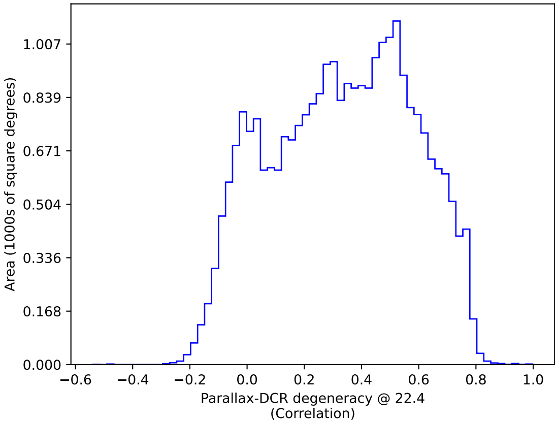
too_ignore_10_1v3.4_10yrs : Parallax-DCR degeneracy @ 22.4
