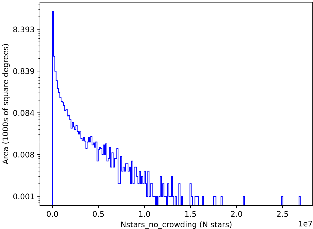
too_ignore_10_1v3.4_10yrs z: Nstars_no_crowding
