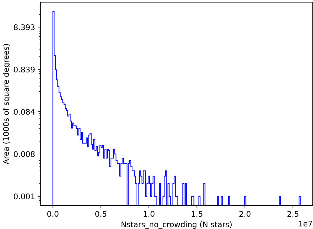
too_ignore_10_1v3.4_10yrs y: Nstars_no_crowding
