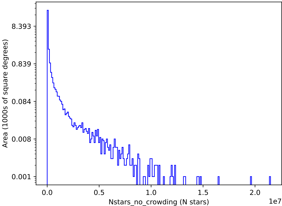
too_ignore_10_1v3.4_10yrs r: Nstars_no_crowding
