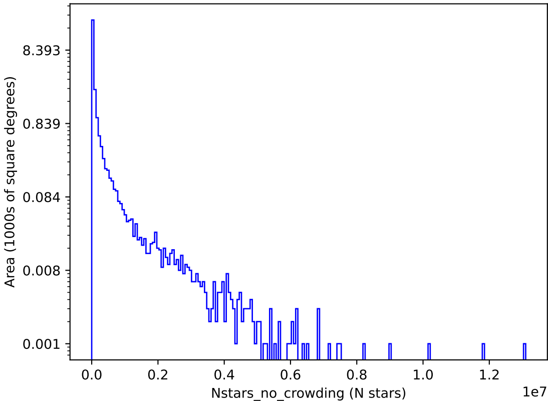
too_ignore_10_1v3.4_10yrs g: Nstars_no_crowding
