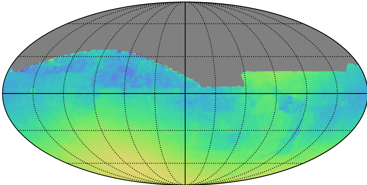
too_ignore_10_1v3.4_10yrs : Normalized Parallax Uncert @ 24.0
