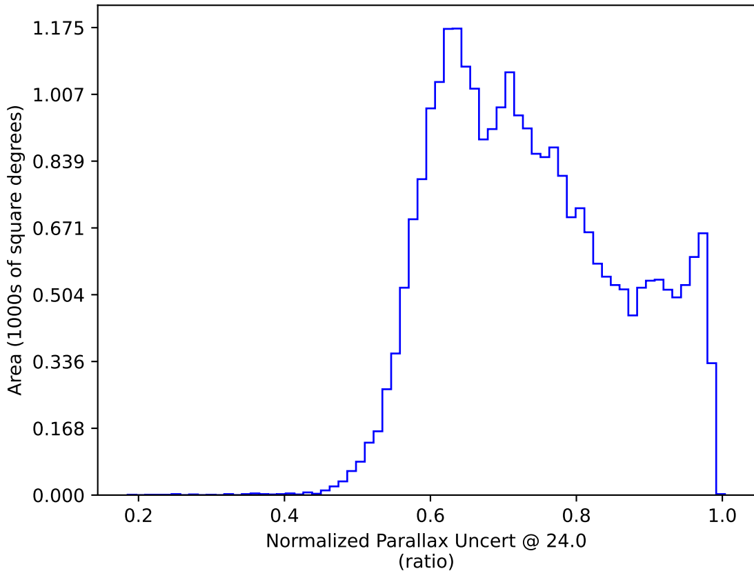
too_ignore_10_1v3.4_10yrs : Normalized Parallax Uncert @ 24.0
