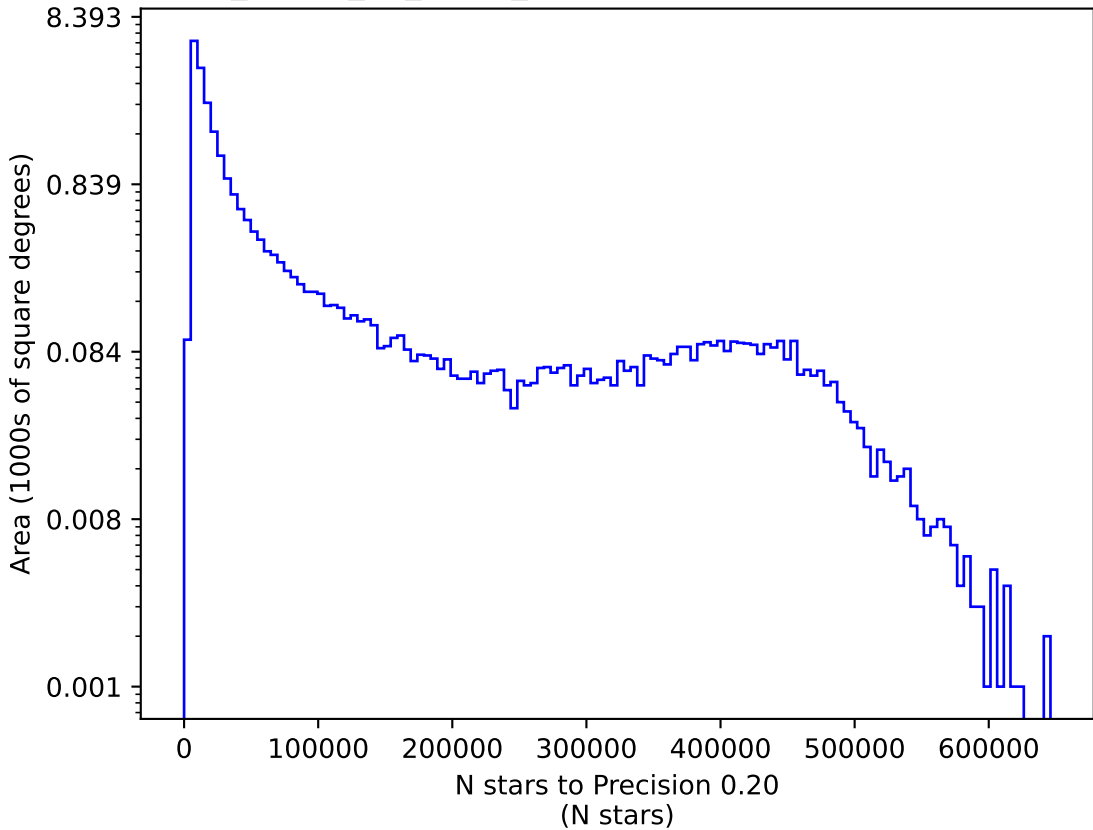
too_ignore_10_1v3.4_10yrs z: N stars to Precision 0.20
