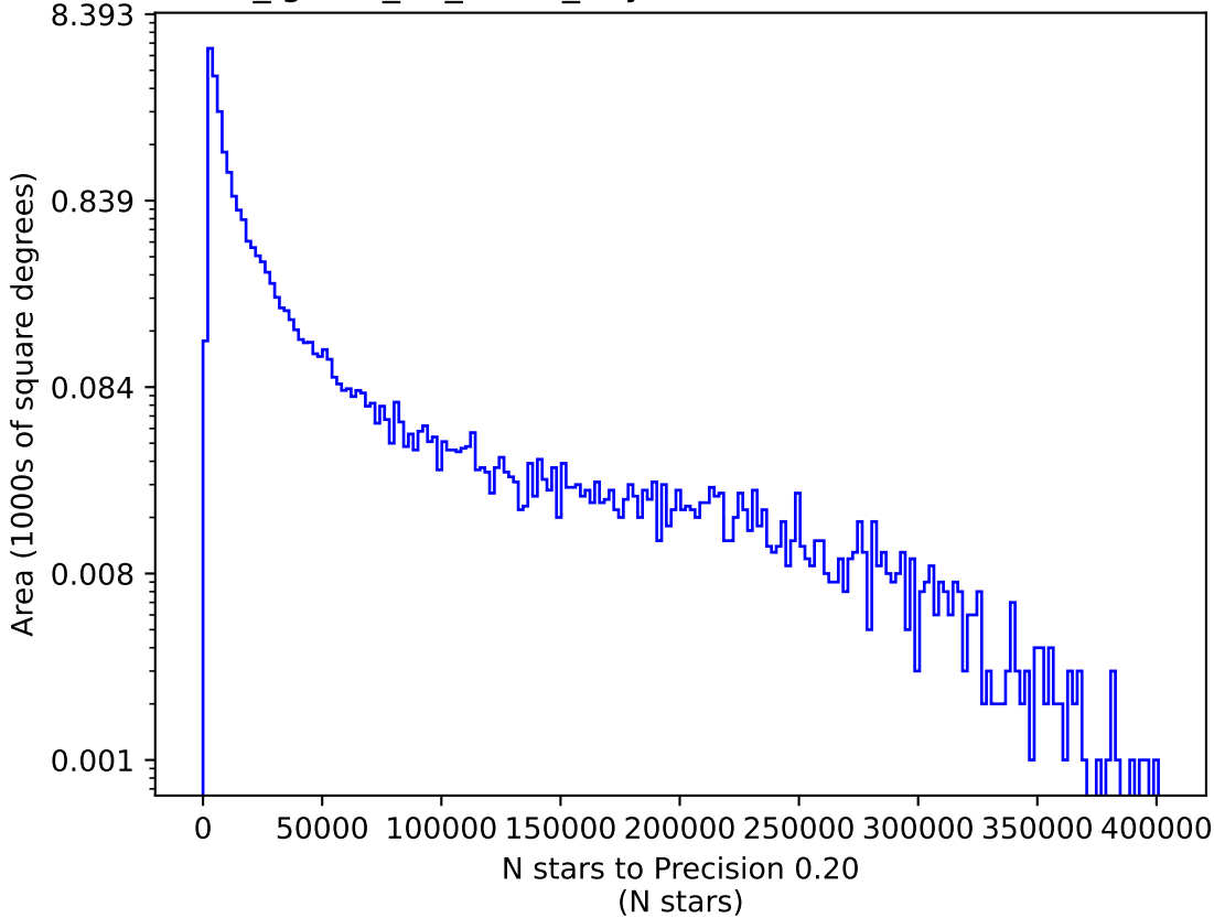
too_ignore_10_1v3.4_10yrs u: N stars to Precision 0.20
