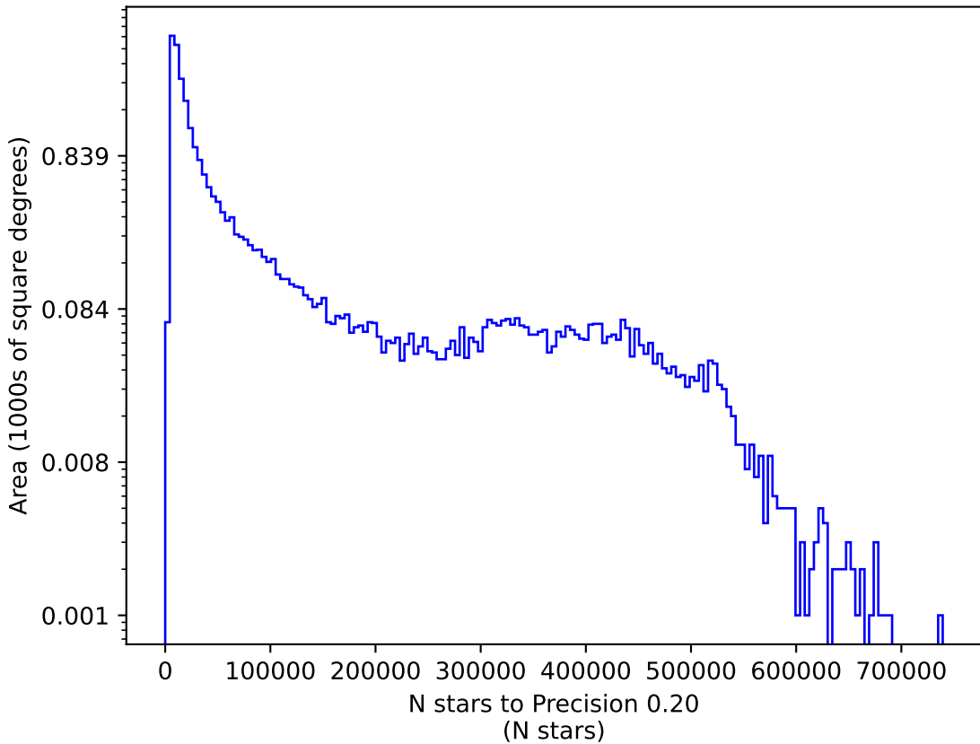
too_ignore_10_1v3.4_10yrs r: N stars to Precision 0.20
