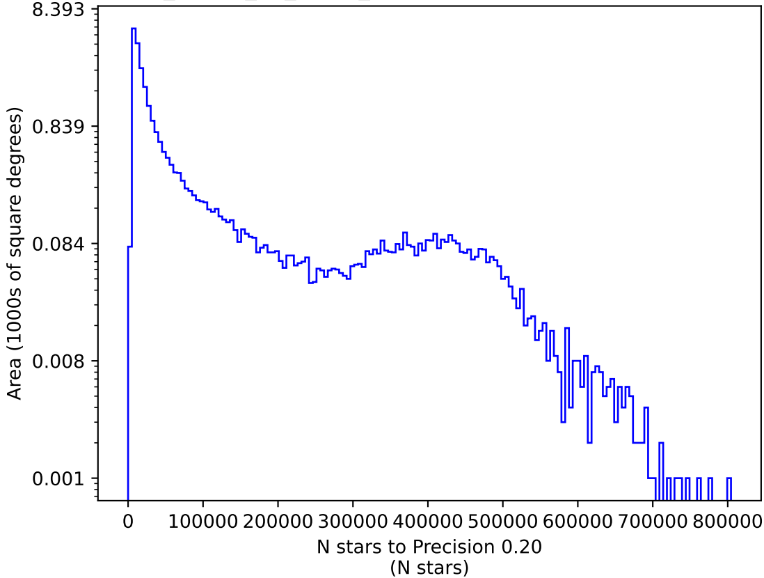
too_ignore_10_1v3.4_10yrs i: N stars to Precision 0.20
