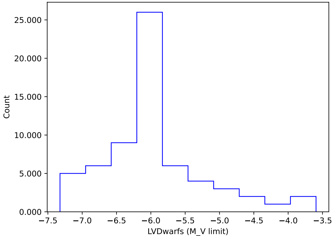
too_ignore_10_1v3.4_10yrs gi: LVDwarfs
