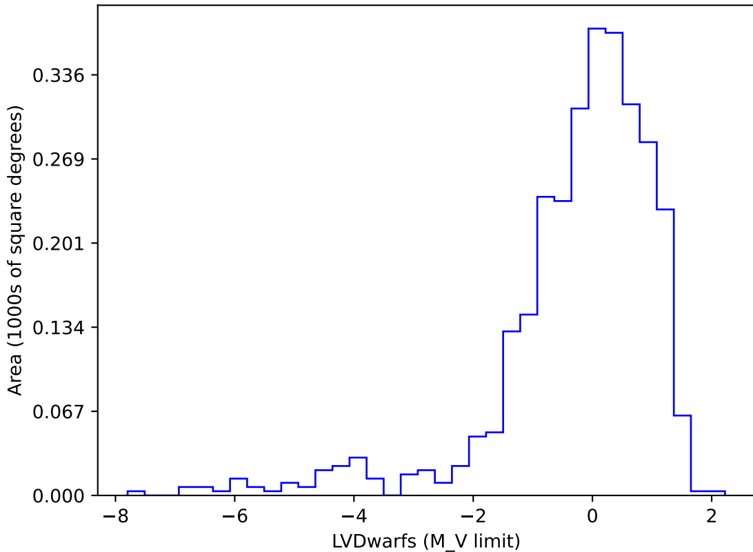
too_ignore_10_1v3.4_10yrs gi SCP: LVDwarfs
