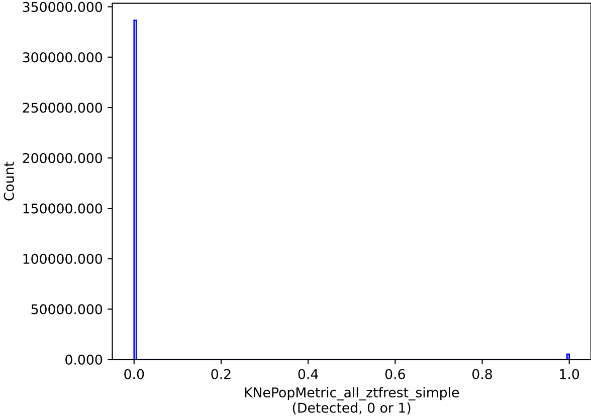
too_ignore_10_1v3.4_10yrs all models: KNePopMetric_all_ztfrest_simple
