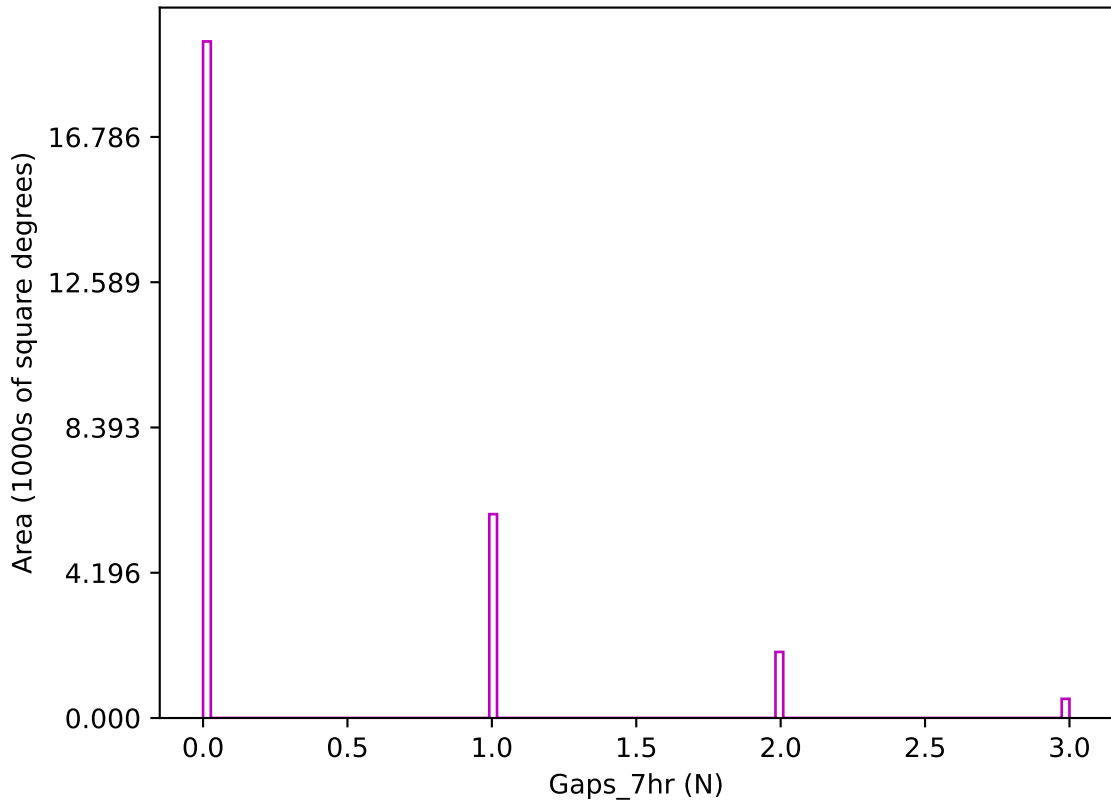
too_ignore_10_1v3.4_10yrs z band: Gaps_7hr
