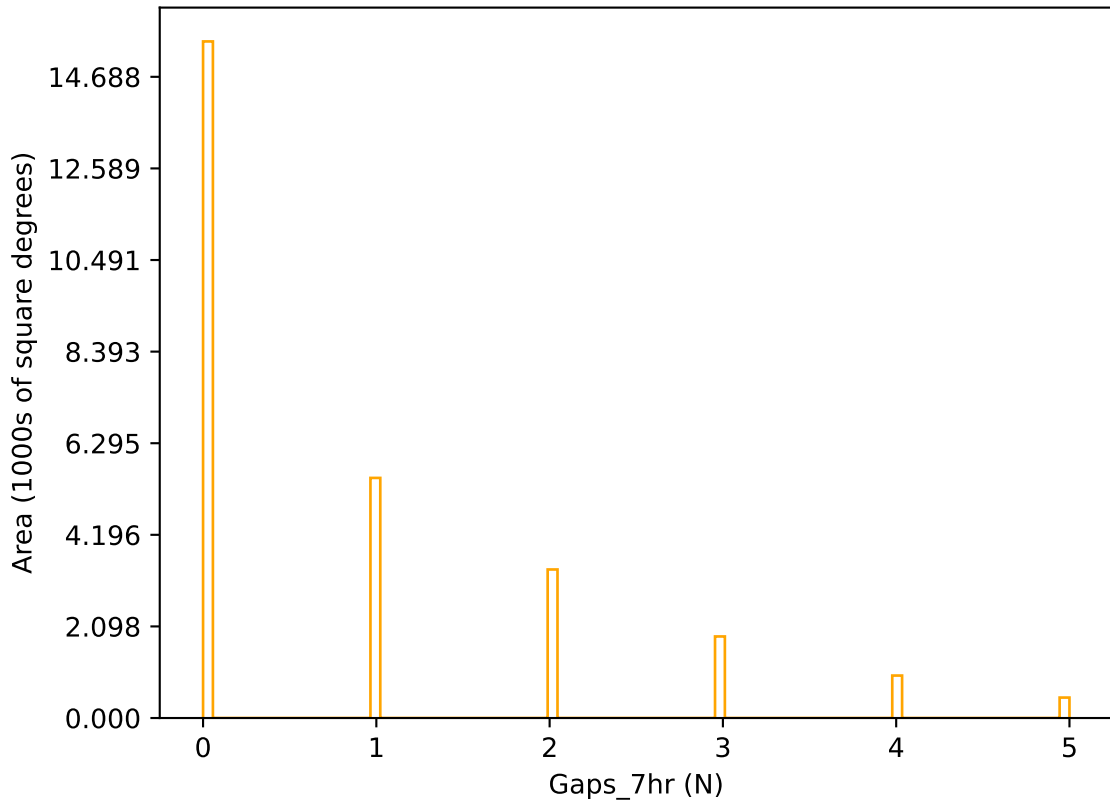
too_ignore_10_1v3.4_10yrs r band: Gaps_7hr
