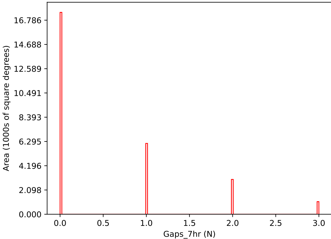
too_ignore_10_1v3.4_10yrs i band: Gaps_7hr
