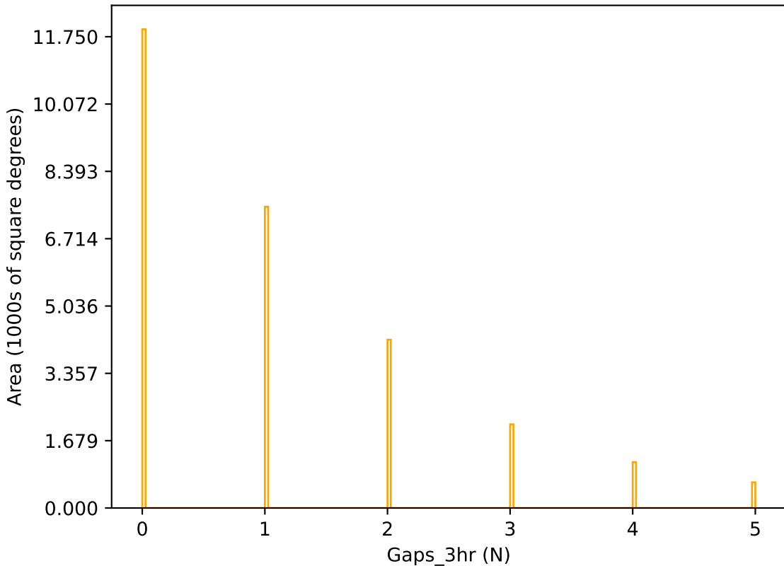
too_ignore_10_1v3.4_10yrs r band: Gaps_3hr
