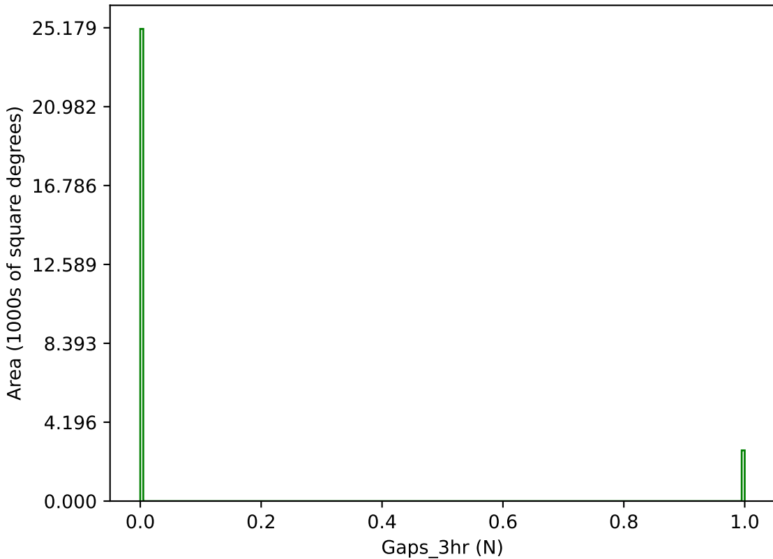
too_ignore_10_1v3.4_10yrs g band: Gaps_3hr
