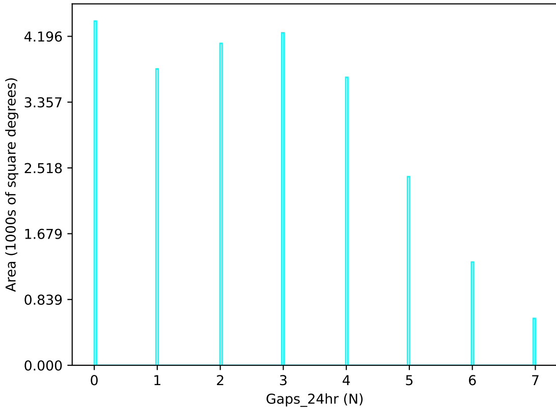
too_ignore_10_1v3.4_10yrs u band: Gaps_24hr
