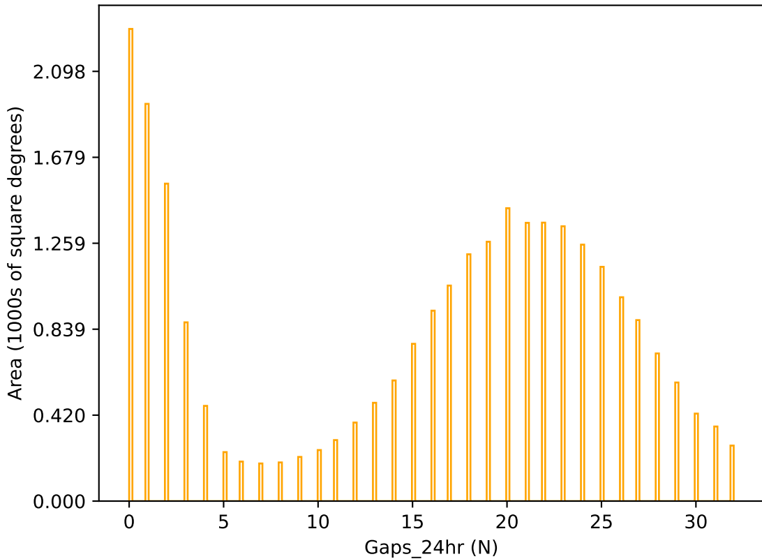
too_ignore_10_1v3.4_10yrs r band: Gaps_24hr
