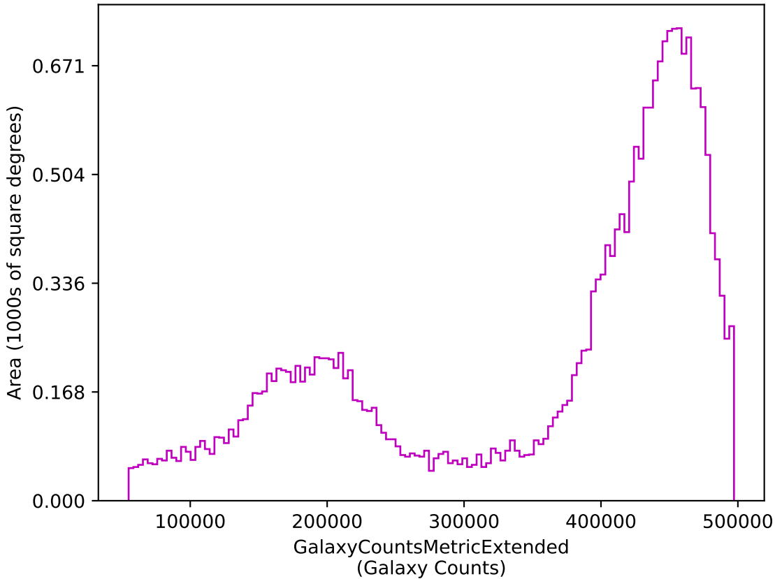
too_ignore_10_1v3.4_10yrs z: GalaxyCountsMetricExtended
