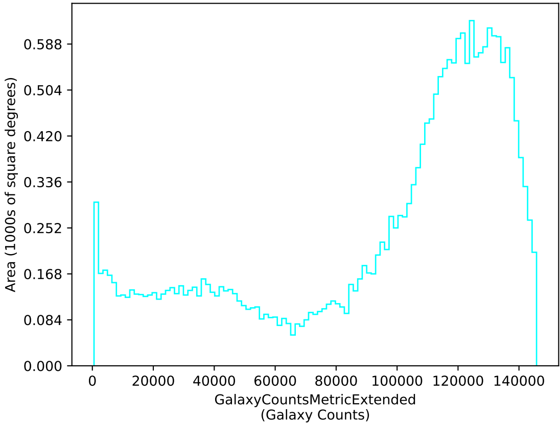
too_ignore_10_1v3.4_10yrs u: GalaxyCountsMetricExtended
