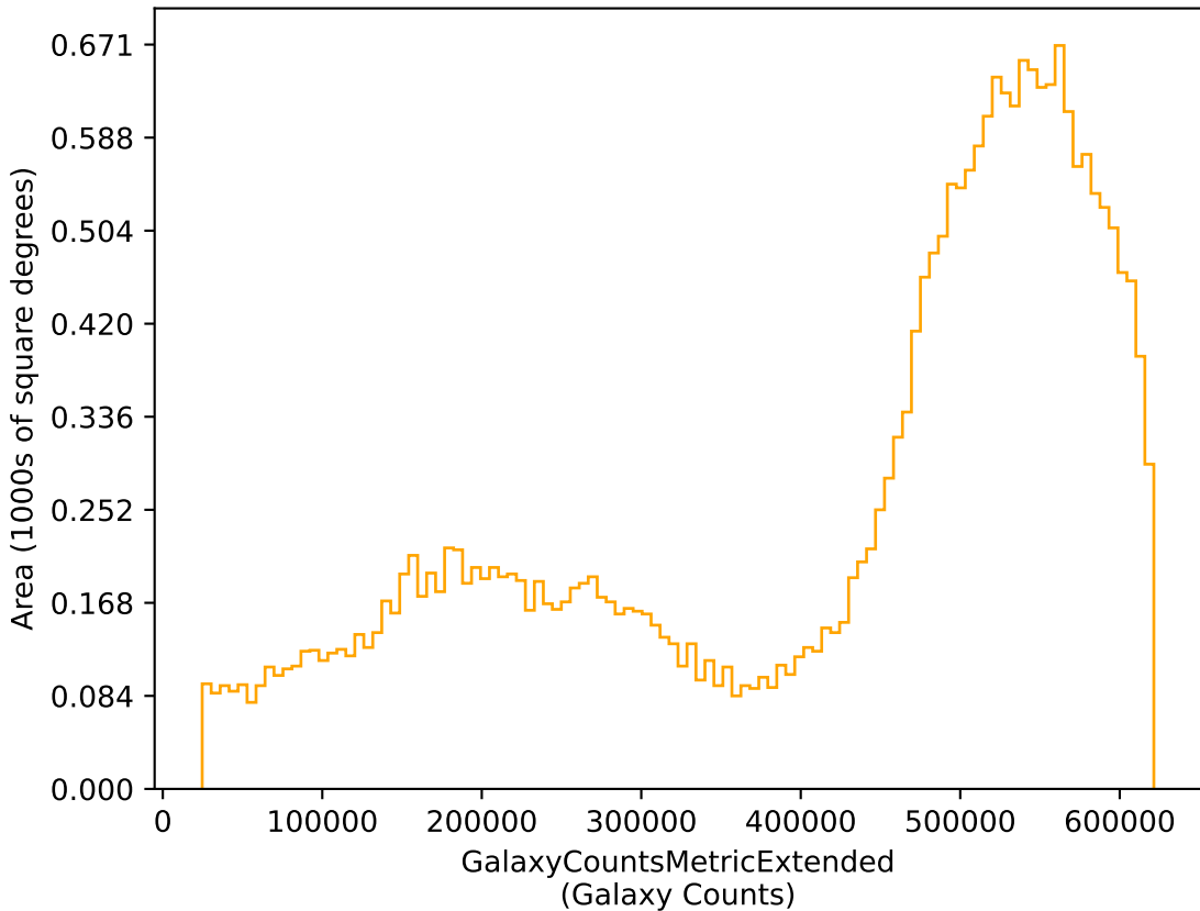
too_ignore_10_1v3.4_10yrs r: GalaxyCountsMetricExtended
