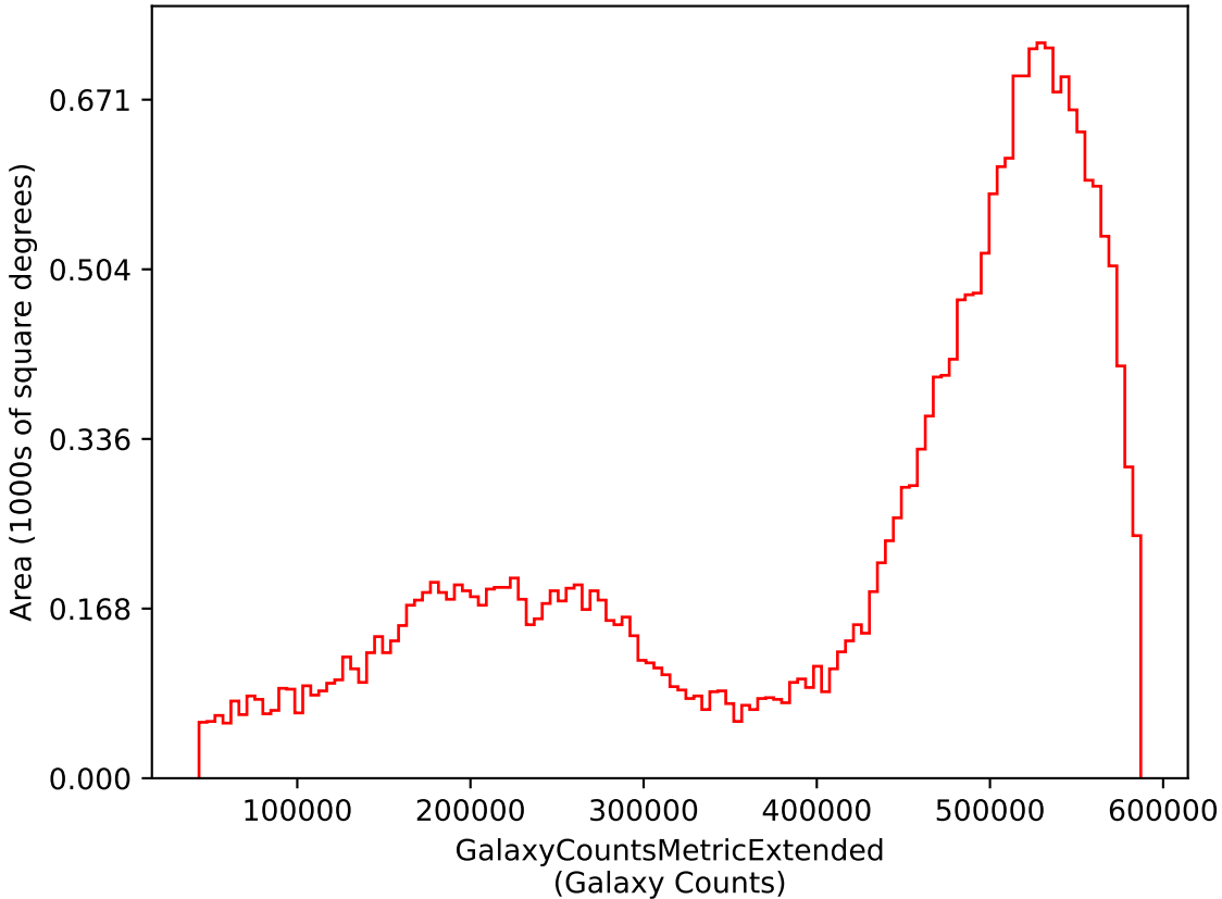
too_ignore_10_1v3.4_10yrs i: GalaxyCountsMetricExtended
