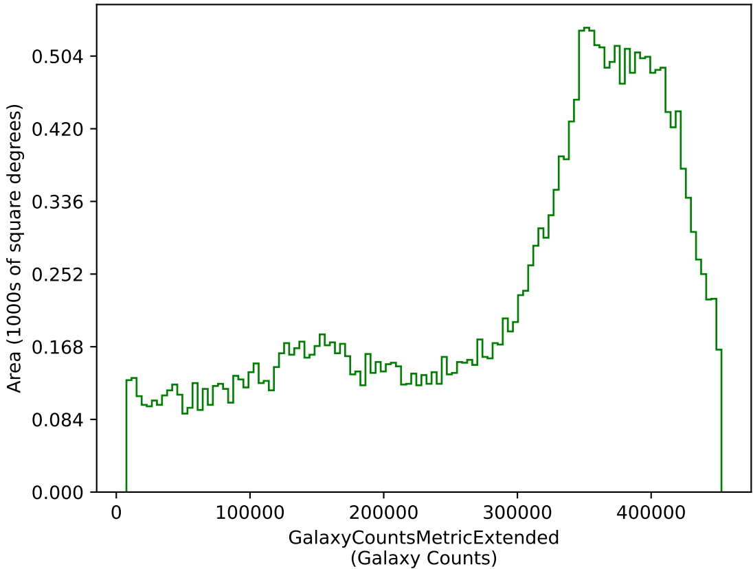
too_ignore_10_1v3.4_10yrs g: GalaxyCountsMetricExtended
