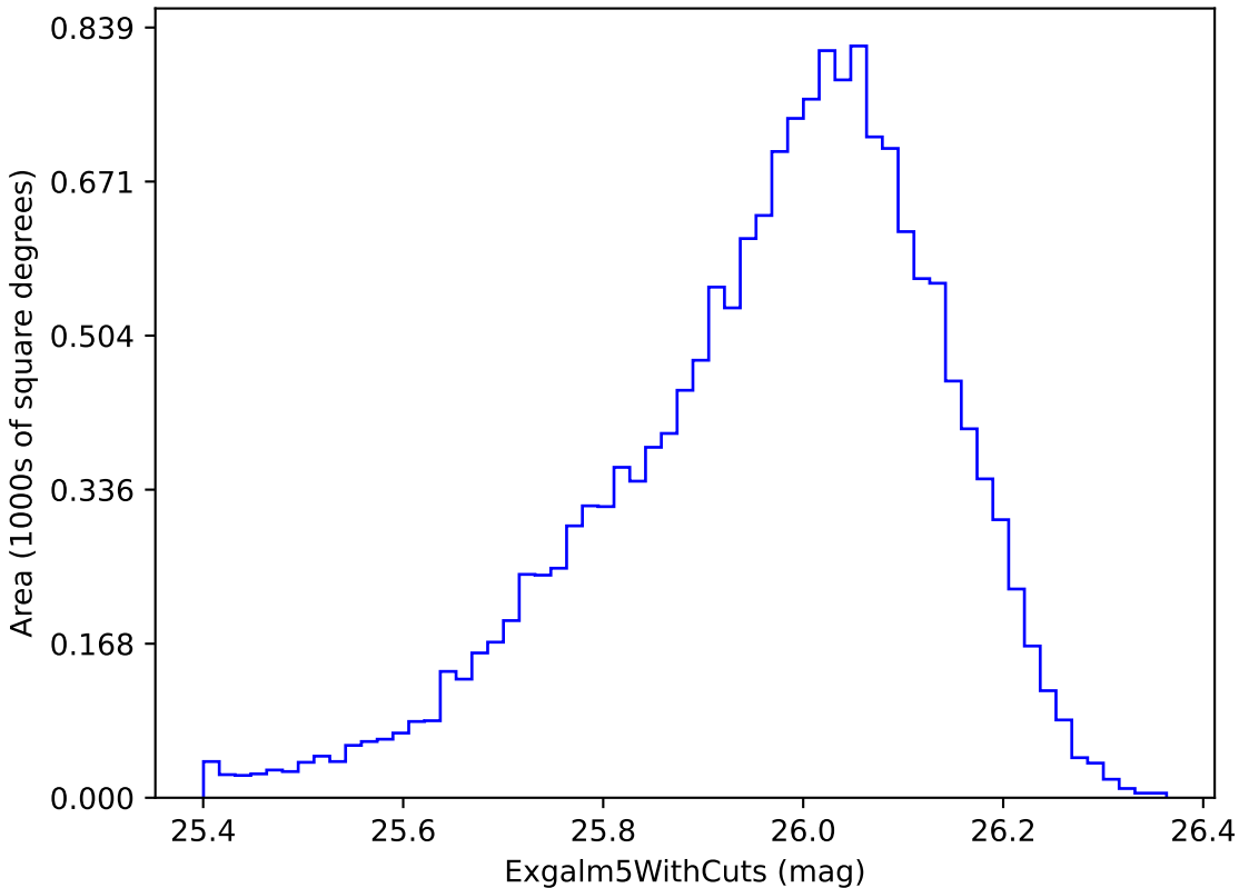
too_ignore_10_1v3.4_10yrs i band non-DD year 4: ExgalM5WithCuts
